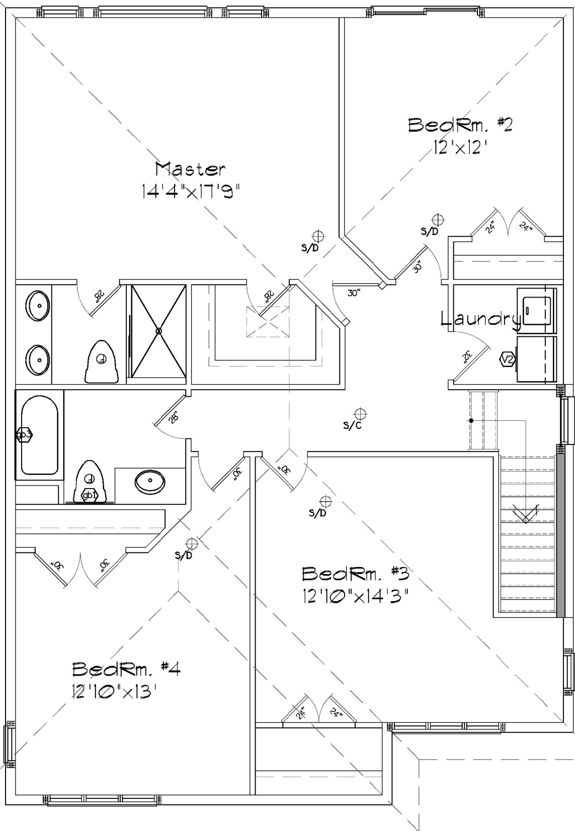
The Stanford Second Floor Plan 1339 sqft
