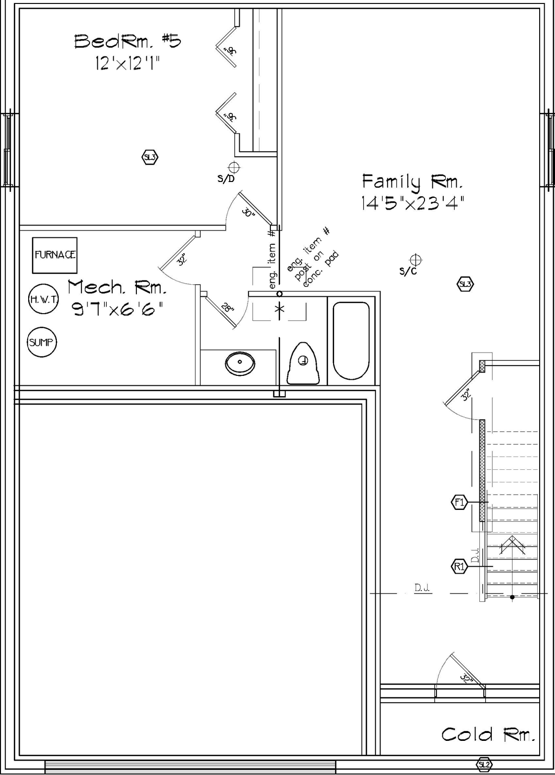
The Stanford Basement Floor Plan 677 sqft
