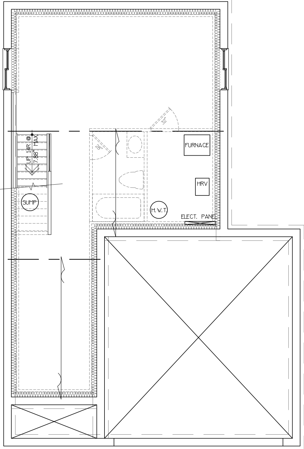
The Princeton Basement Floor Plan
