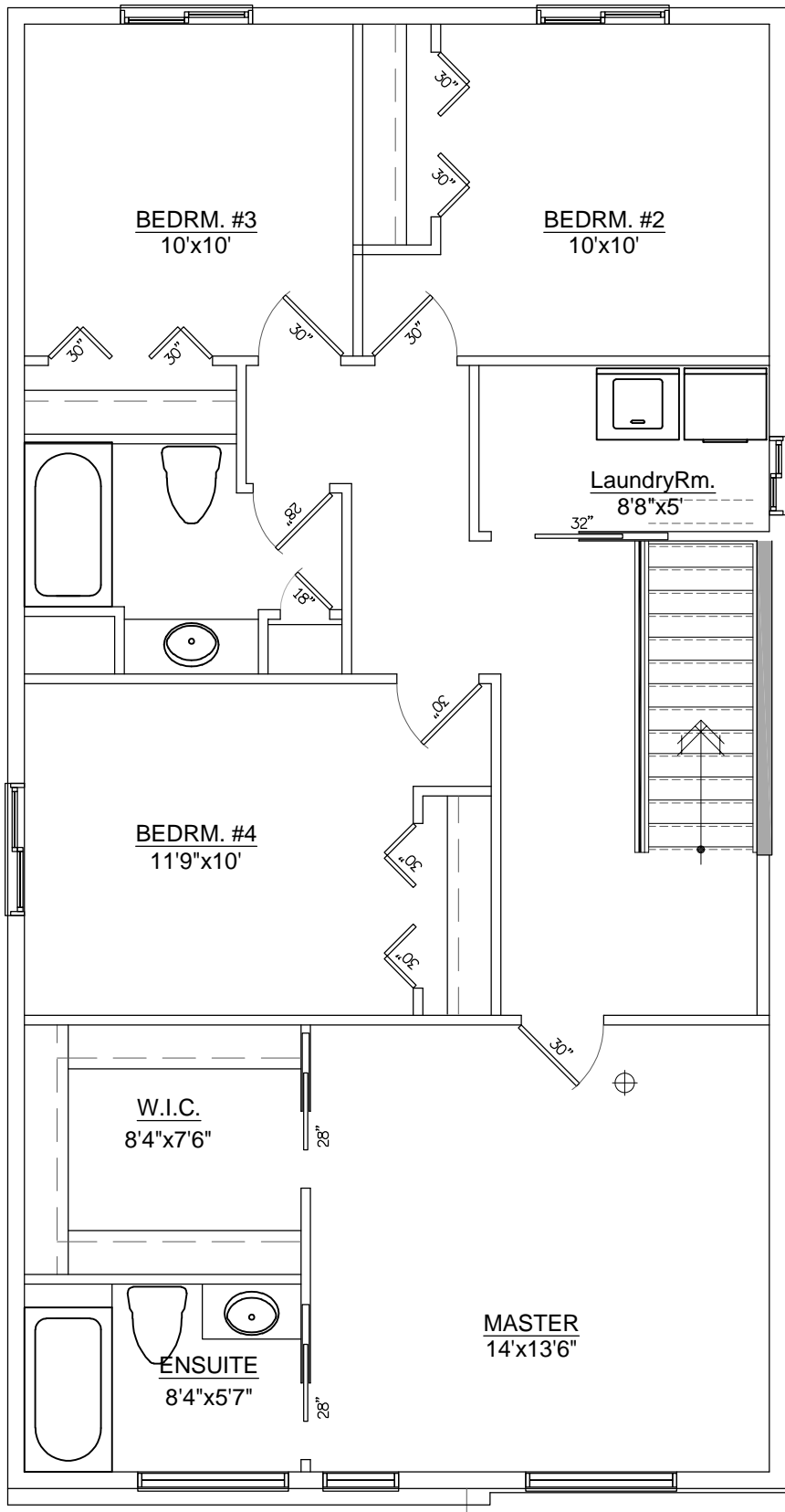
The McMaster Second Floor Plan 1065 sqft
