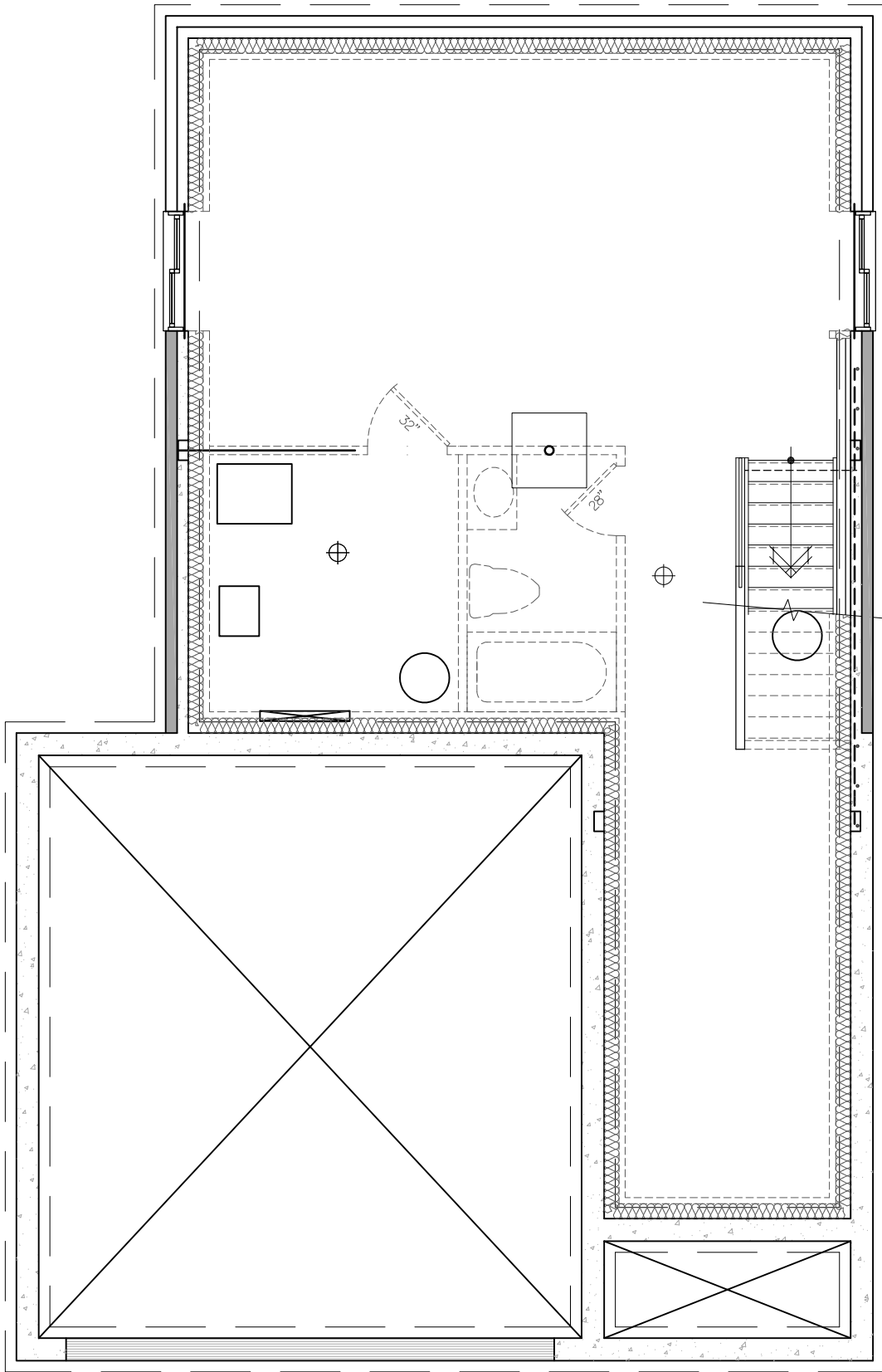
The McMaster Basement Floor Plan
