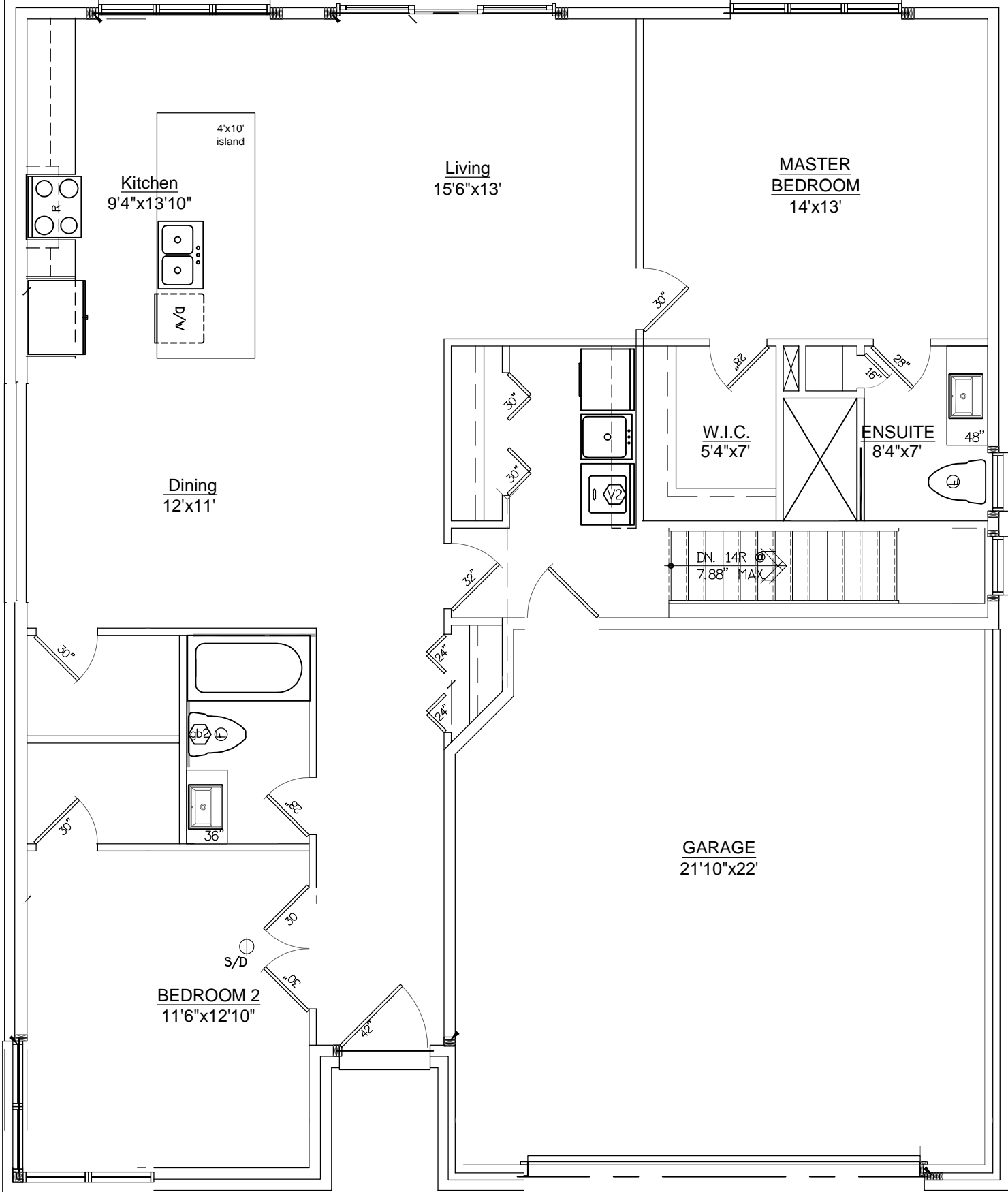
The Cornell Main Floor Plan 1451 sqft
