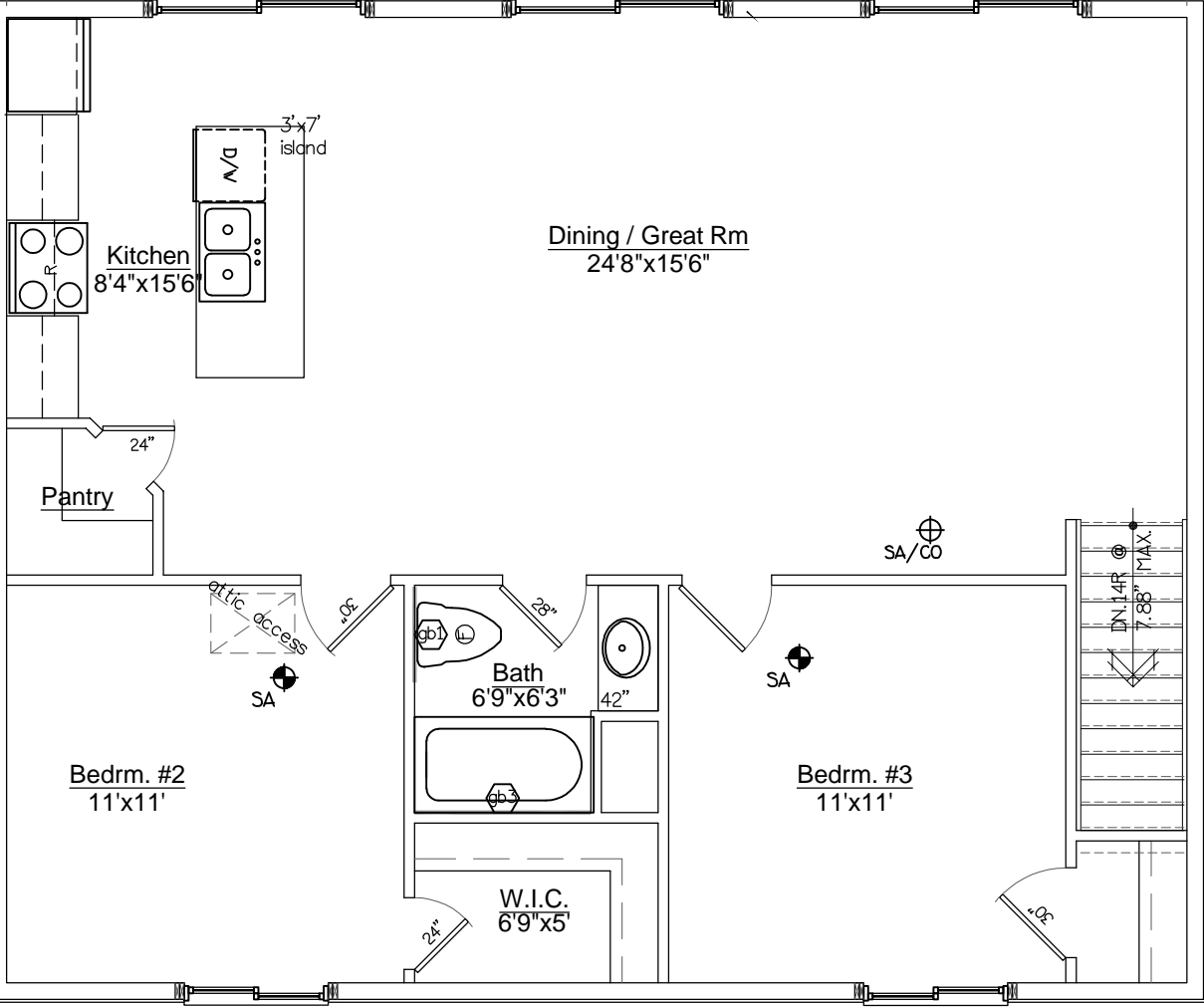
The Boswell Second Floor Plan 952 sqft
