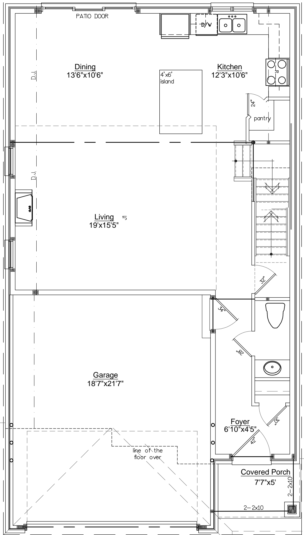
The Basit Main Floor Plan 892 sqft
